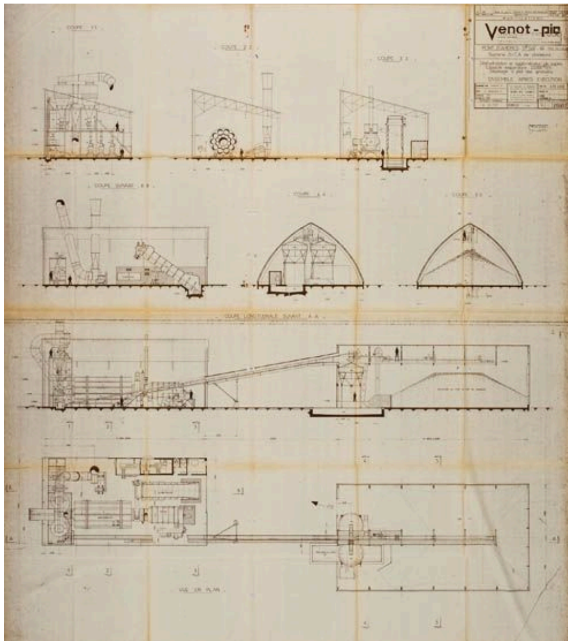
Plan technique Venot-Pic. (AD Seine-et-Marne, 256J4)
